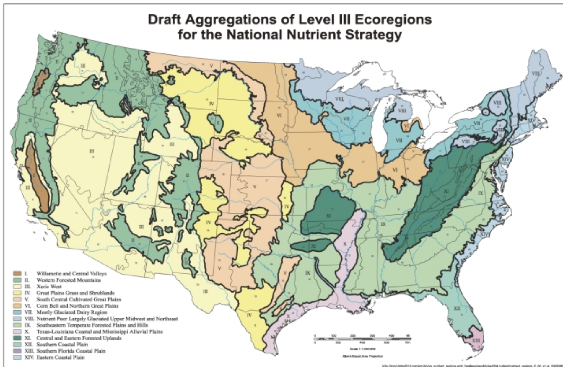
Figure 4. Fourteen nutrient ecoregions as delineated by Omernik (2000). Ecoregions were based on geology, land use, ecosystem type, and nutrient conditions.
